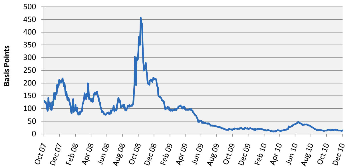
Figure 37: TED Spread 463
