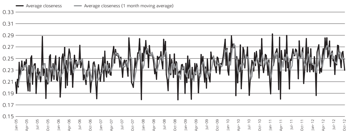
Figure 12. Average Closeness
