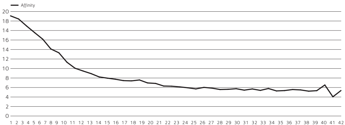
Figure 9. Affinity Function
