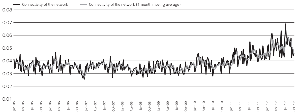
Figure 15. Connectivity
