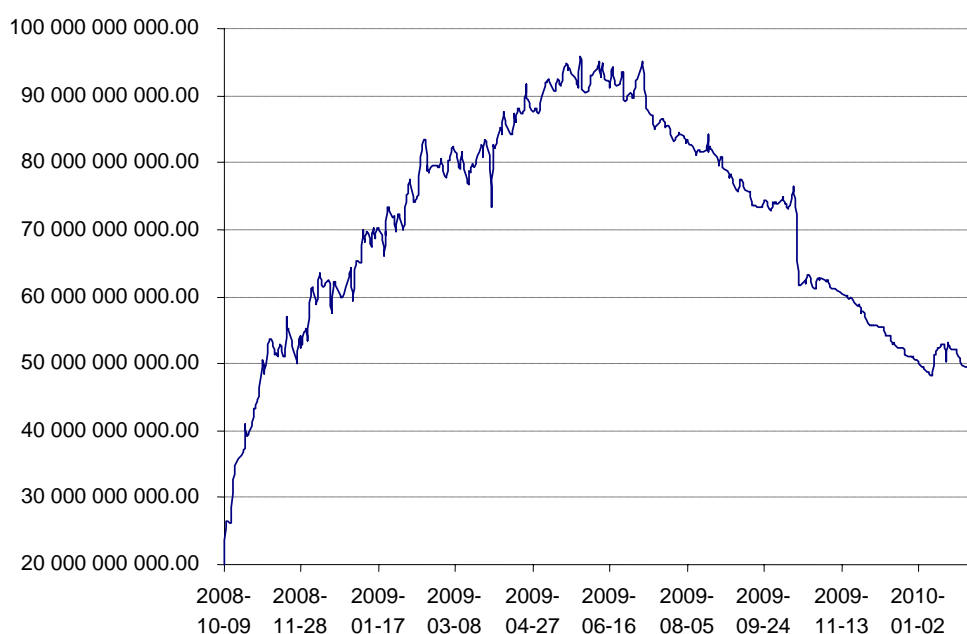
Fig. 1: Trend in the volume of Dexia bonds covered by the guarantee
